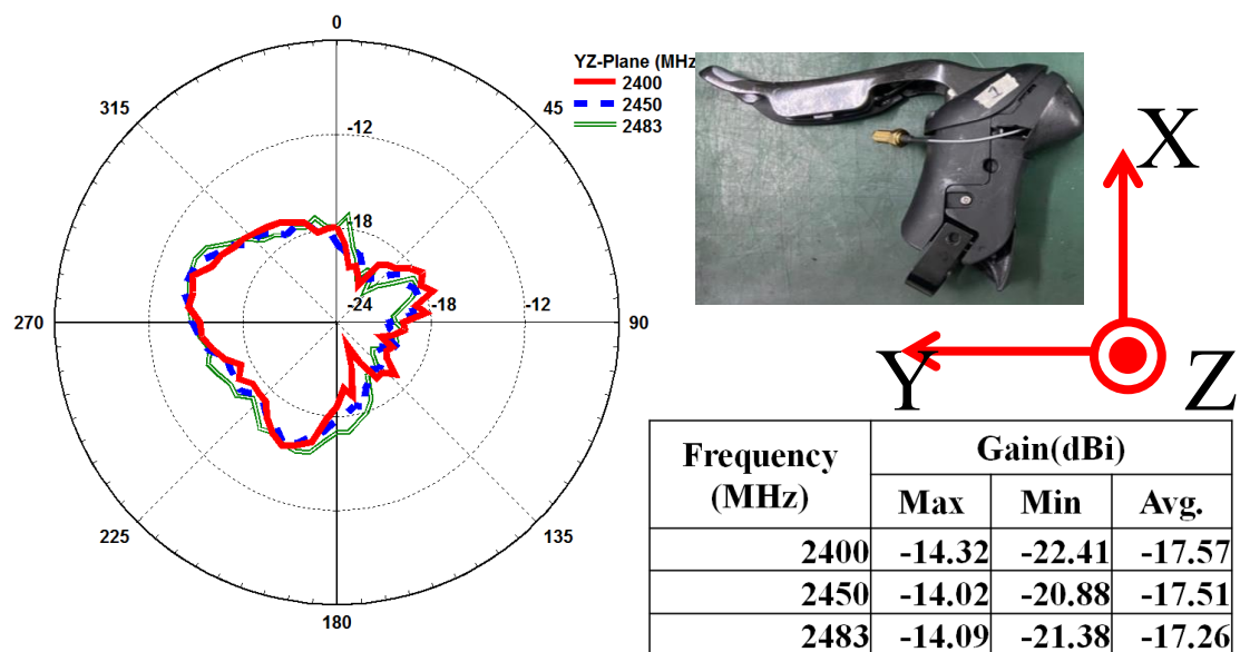
Radiation pattern_R and gain in the \Phi=90^\circ with housing
