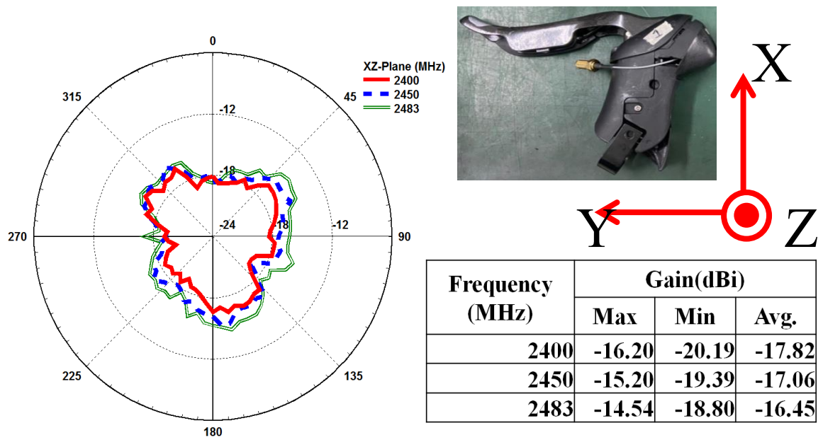
Radiation pattern_R and gain in the \Phi=0^\circ with housing
