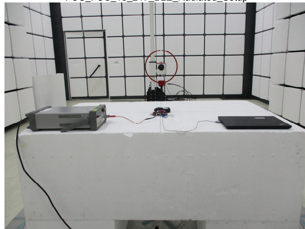
FCC_FCC_15_247_BLE_Radiated_Setup
