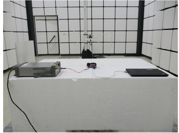
FCC_FCC_15_247_BLE_Radiated_Setup
