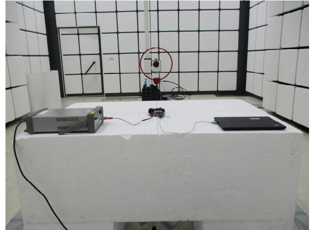
FCC_FCC_15_247_BLE_Radiated_Setup
