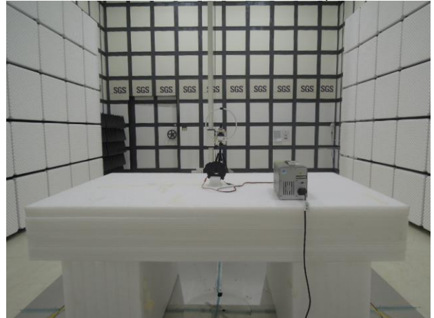
FCC_15_247_ANT+_Radiated_Setup
