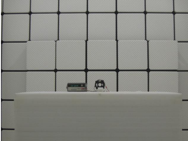
FCC_15_247_ANT+_Radiated_Setup
