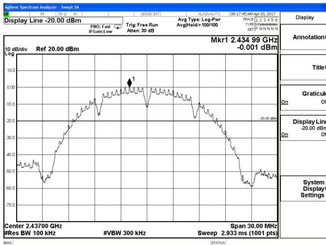
802.11b_Middle Channel
