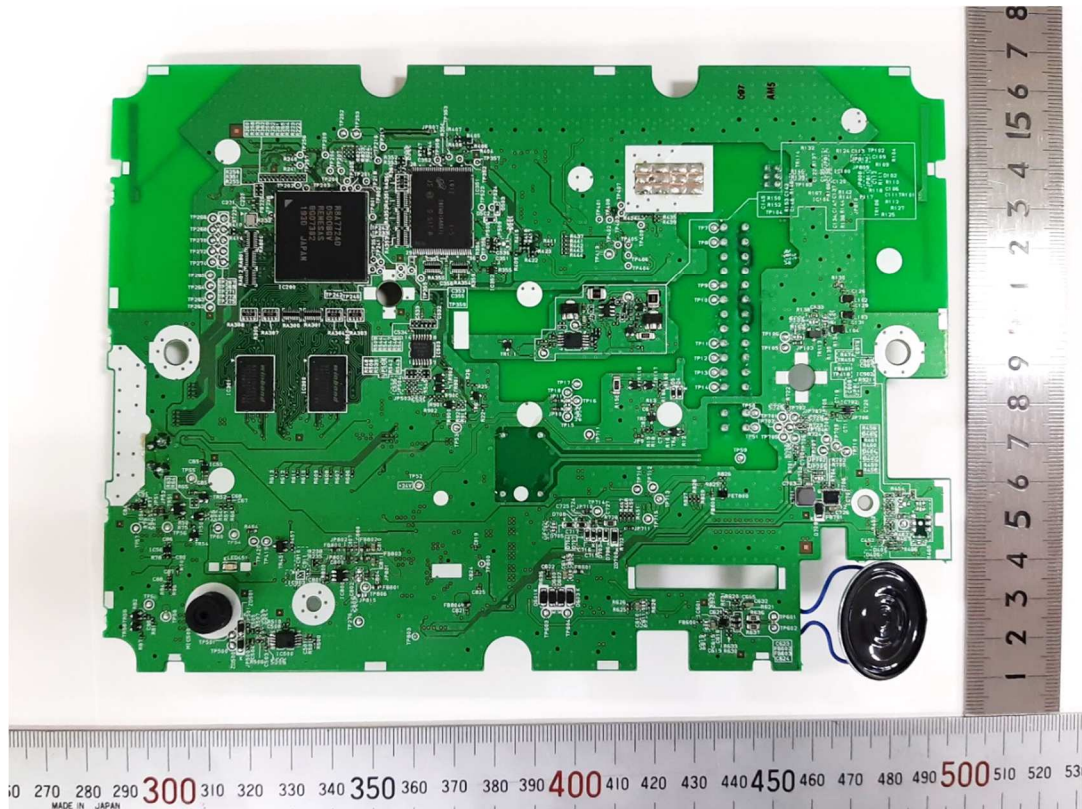
Around W-LAN Module [Side-A]
