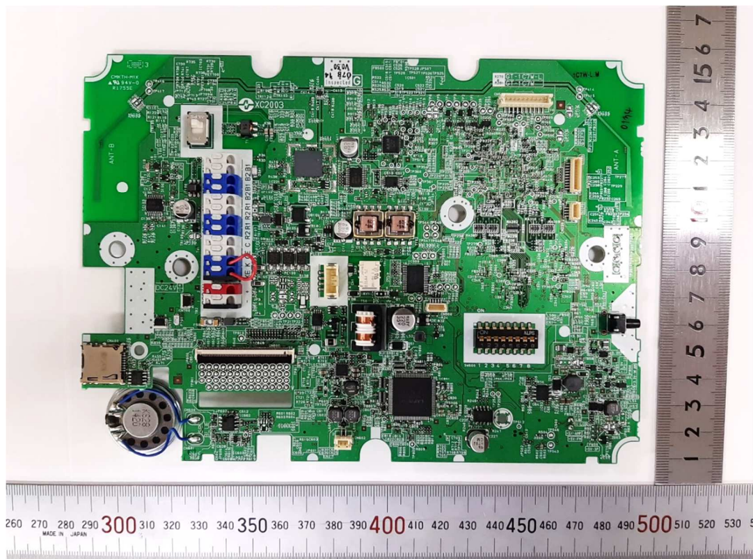
XC2003 [Side-A]
