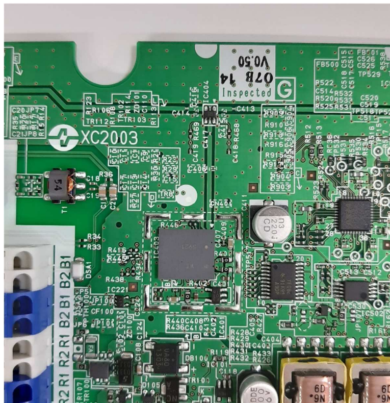
Around W-LAN Module [Side-A]
