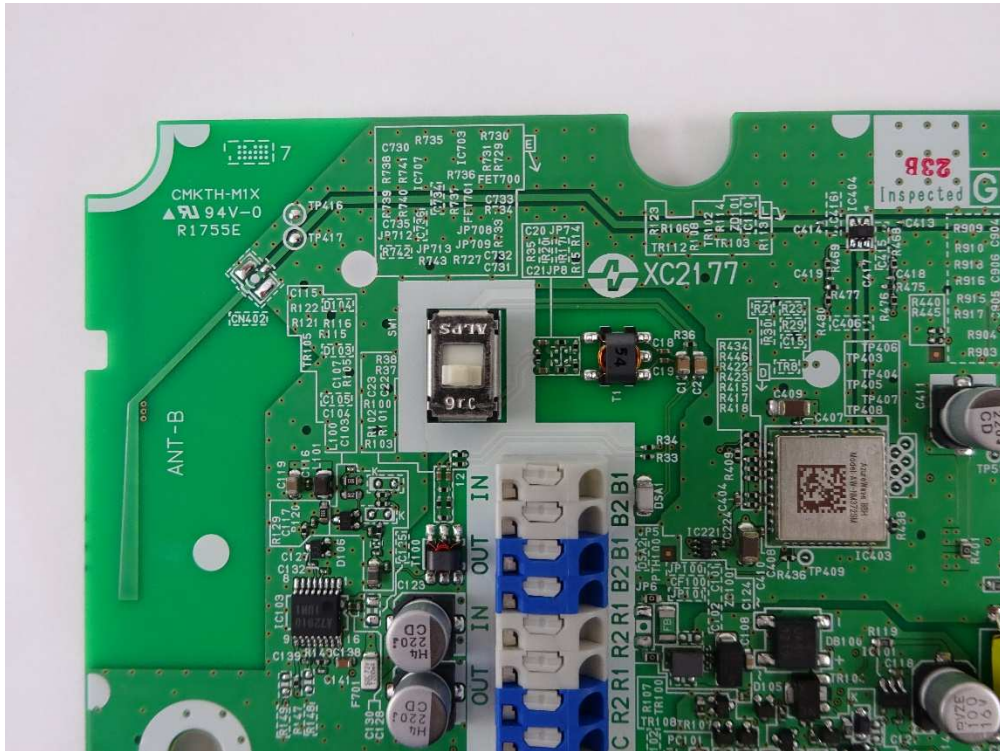
Internal Photos of GT-1C7W-L V2 Around ANT-B [Side-A]
