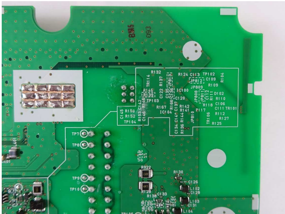
Around ANT-B [Side-B]
