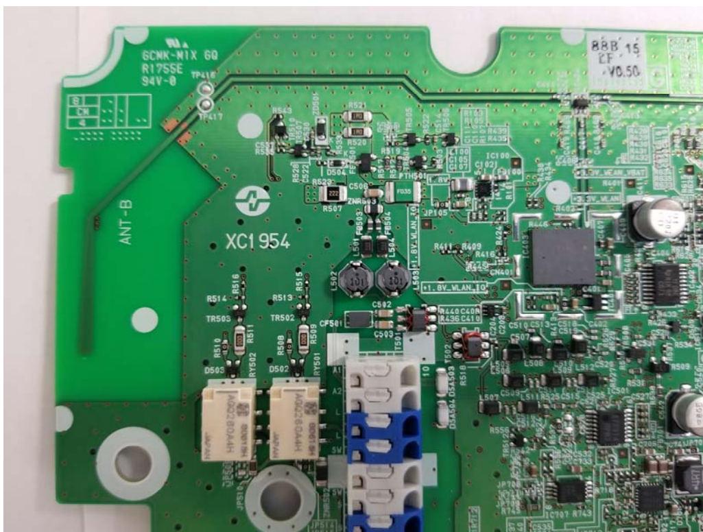
Antenna B Close-up Front
