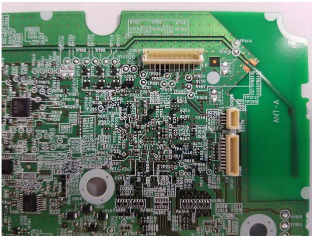
Antenna A Close-up Front
