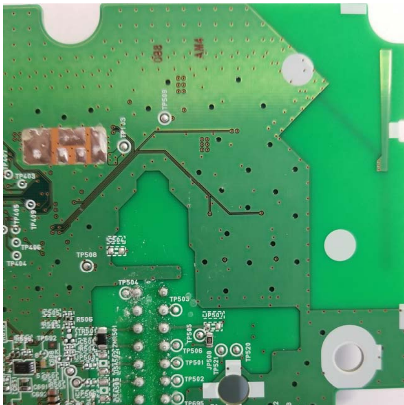
Antenna B Close-up Rear
