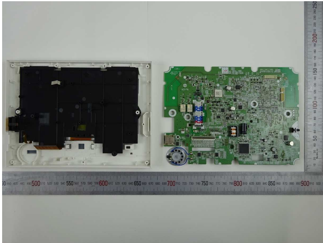
Internal Photos of JO-1MDW V2
