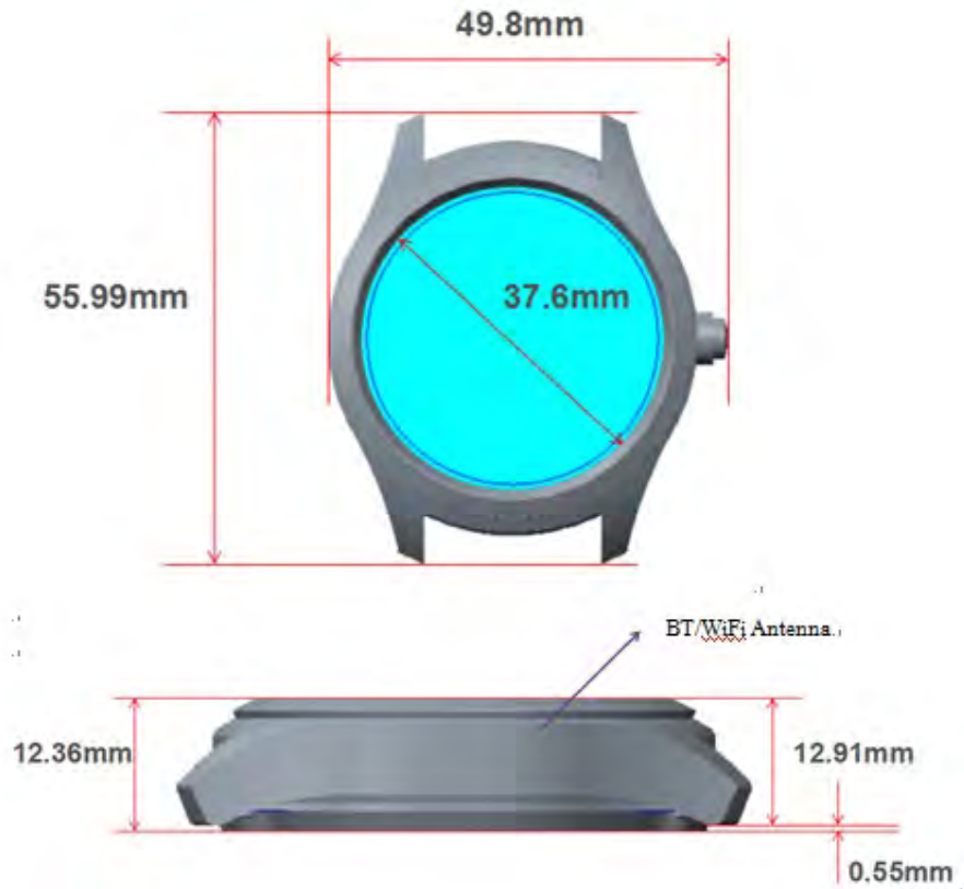
Fig.6 Antenna location
