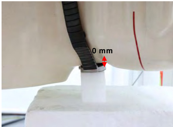
Fig.5 Configuration 3: remove the one side's watchband and make the watch's back touch against the neck phantom area
