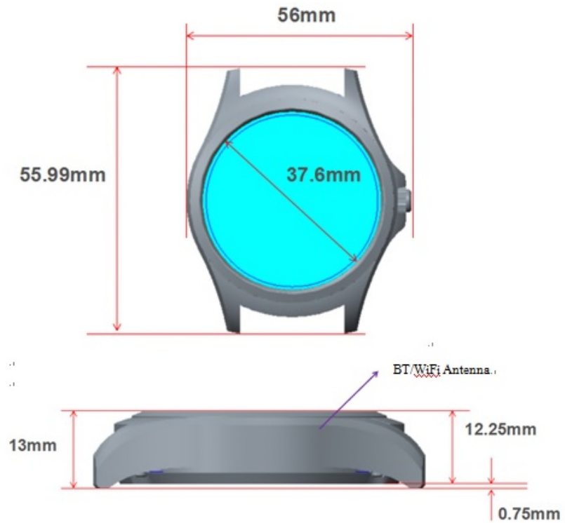
Antenna location (front view)
