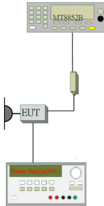
Fig.2-3 Conducted Emission (Antenna Port) Configuration
