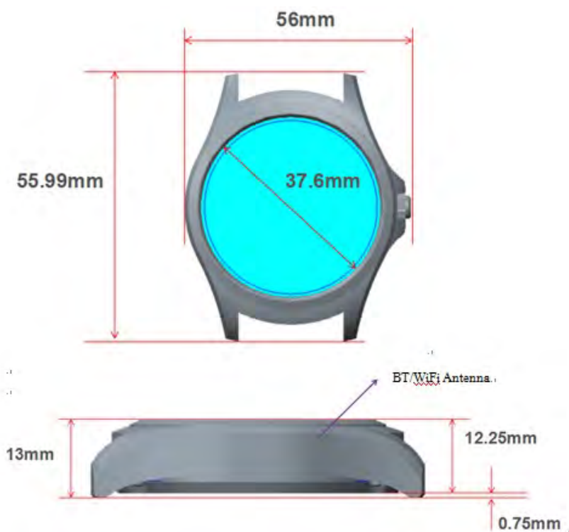
Fig.6 Antenna location
