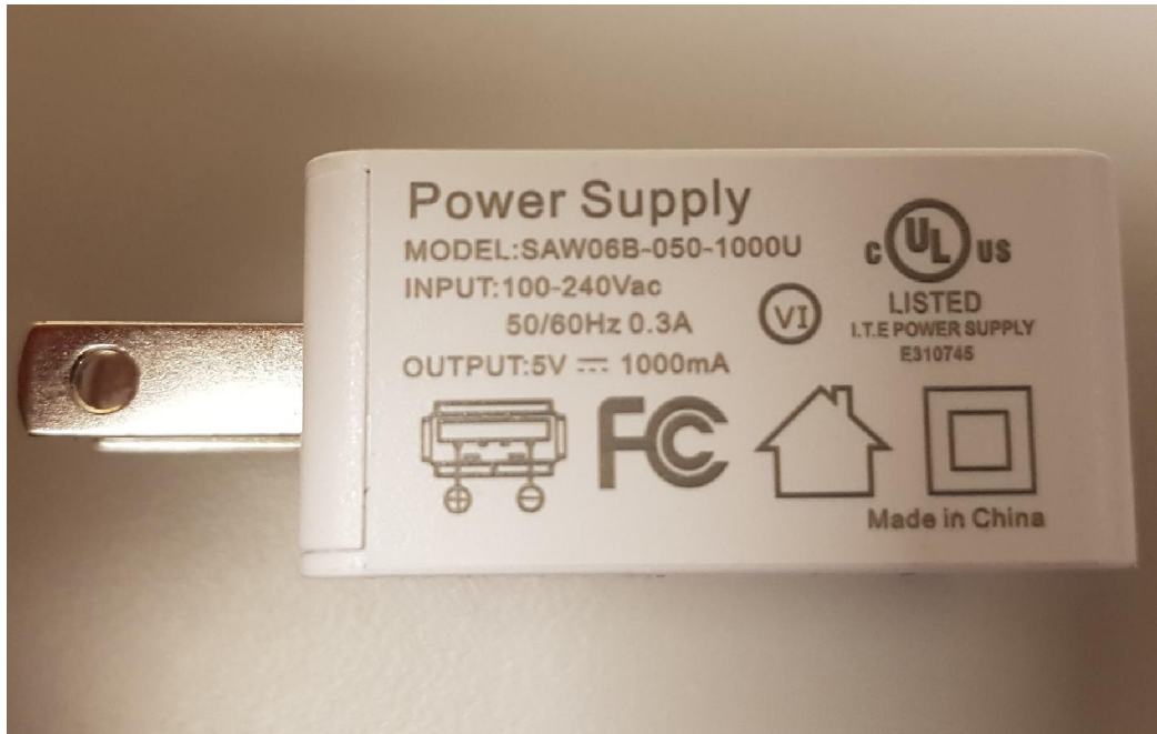
Power supply
