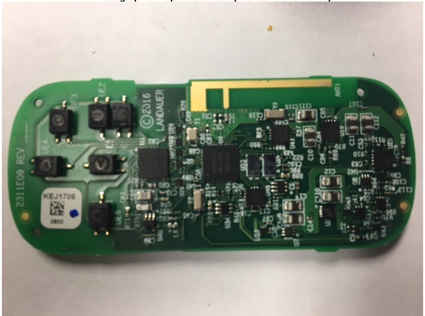
Photograph of Top Side of PCB (with covers removed)
