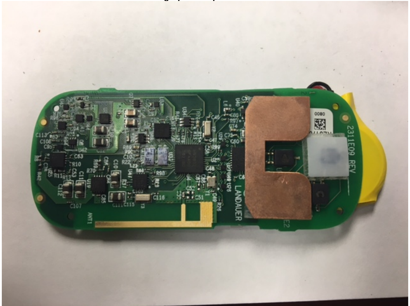
Photograph of Top Side of PCB
