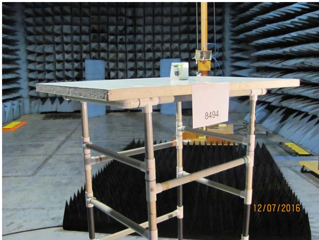
Photograph of BW Test Setup
