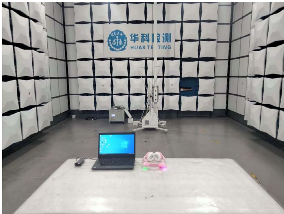
Model: HKLEDBTHP1 Radiated Emissions
