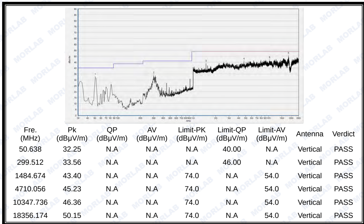
(Plot B.3: Antenna Vertical, 30MHz to 25GHz)
