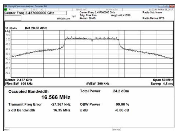
Channel 06 (2437MHz)
