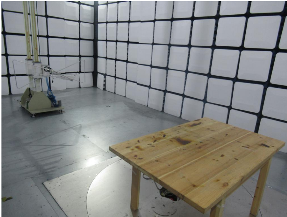
FCC ID: 2ALON-VXBLEBEACOM Photo of Radiation Emission Test
