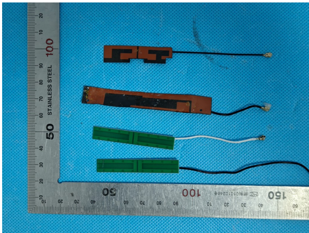
ANTENNA CLOSE-UP PHOTO-6
