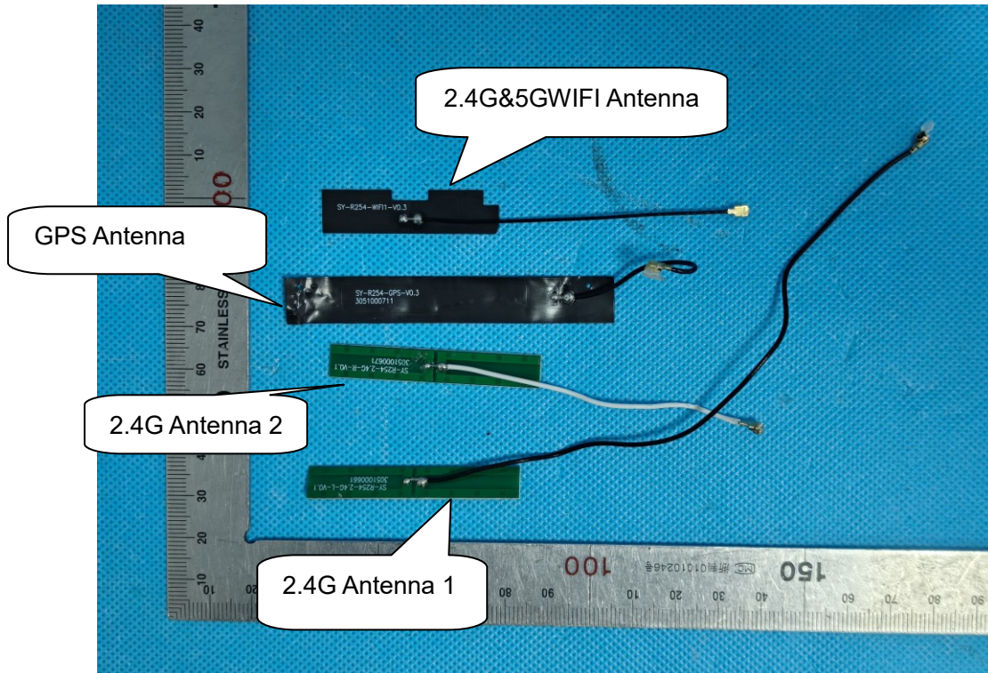
ANTENNA CLOSE-UP PHOTO-6
