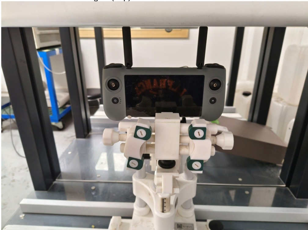
Edge 1 (Top) antenna rotates 180° 0mm
