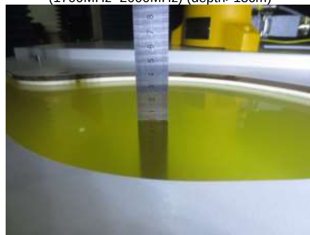
Fig. 9.6 Photo of Liquid Height for Body SAR (2000MHz~2600MHz)(depth>15cm)
