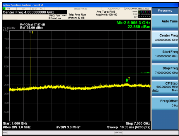
PCS 1900-MCH
