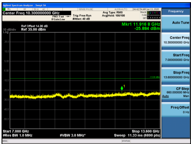
PCS 1900-MCH
