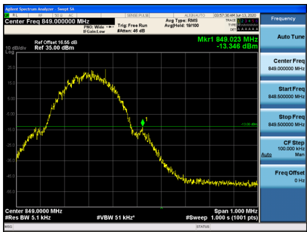
GSM 850-HCH-GSM
