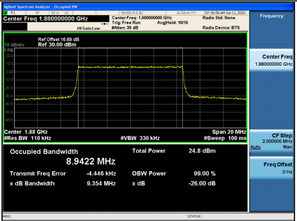
MCH_16QAM_50RB#0
