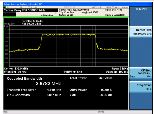
MCH_16QAM_15RB#0
