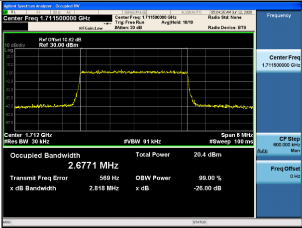
LCH_16QAM_15RB#0
