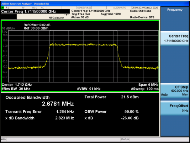
LCH_QPSK_15RB#0
