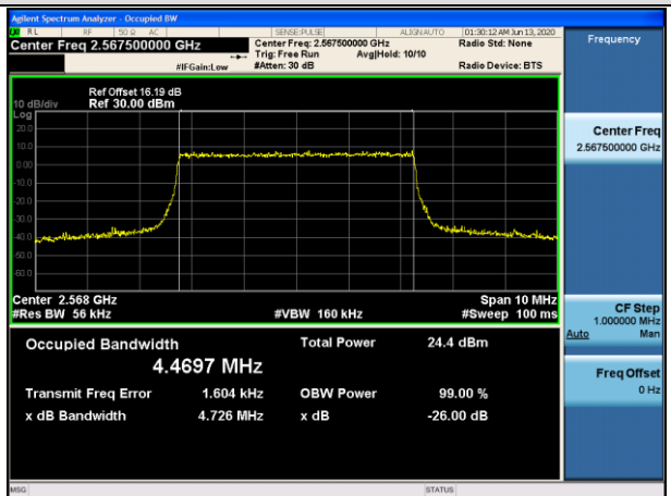
HCH_16QAM_25RB#0
