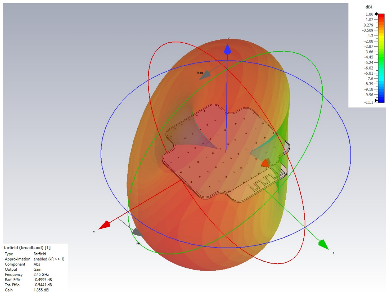
3D Antenna Radiation Diagram (2450MHz)
