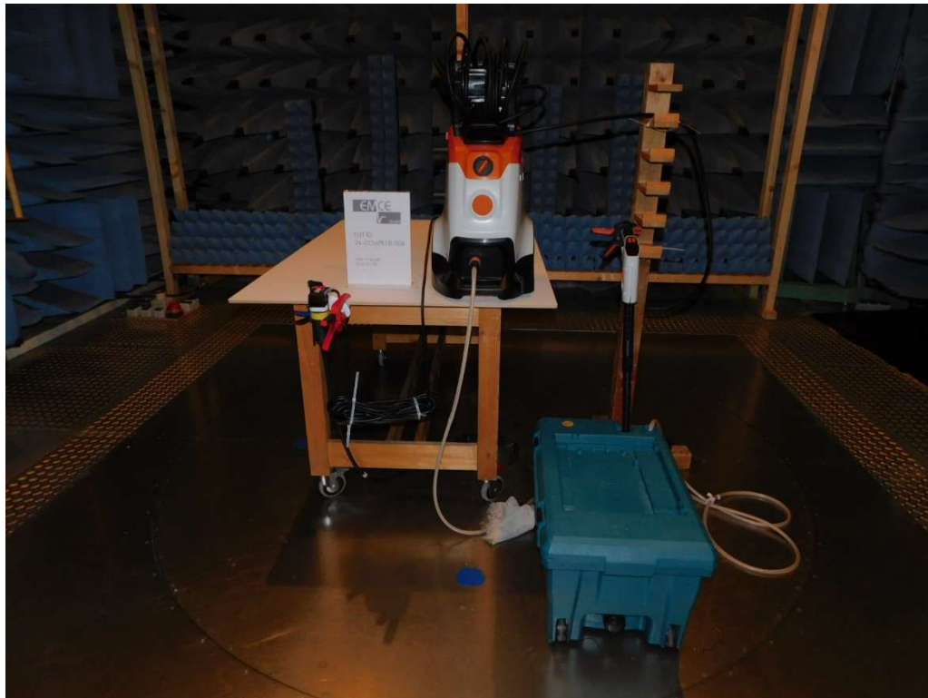
Pre-test setup – SAC [30 – 1000 MHz]
