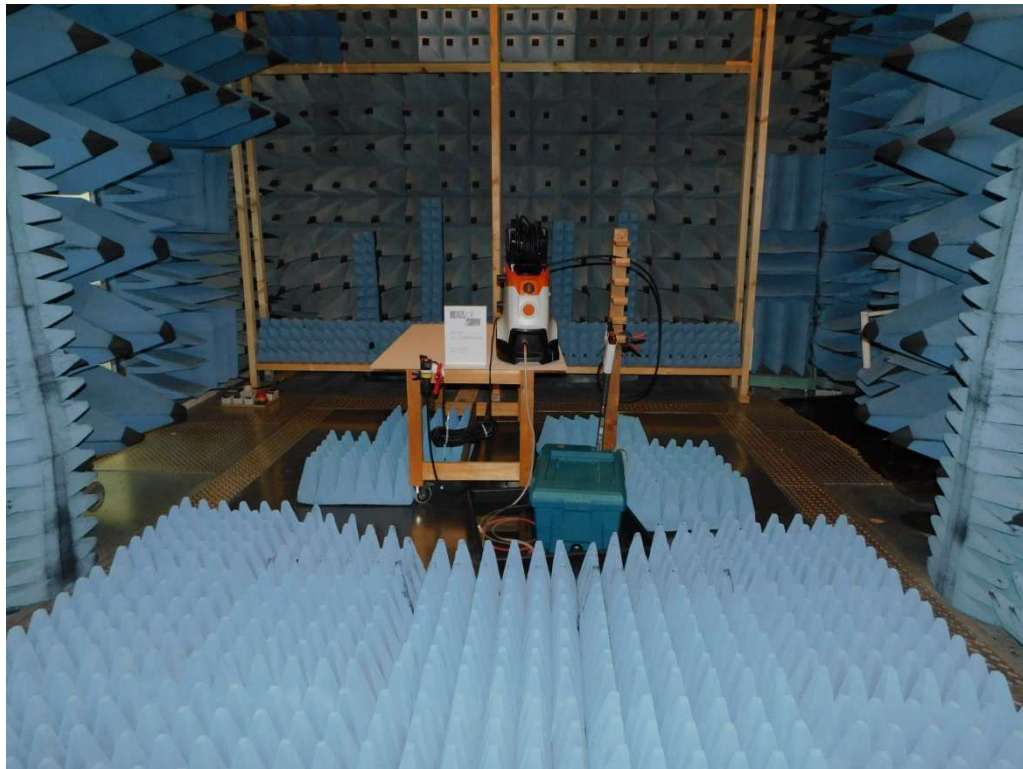
Final test setup – SAC [1 – 5 GHz]
