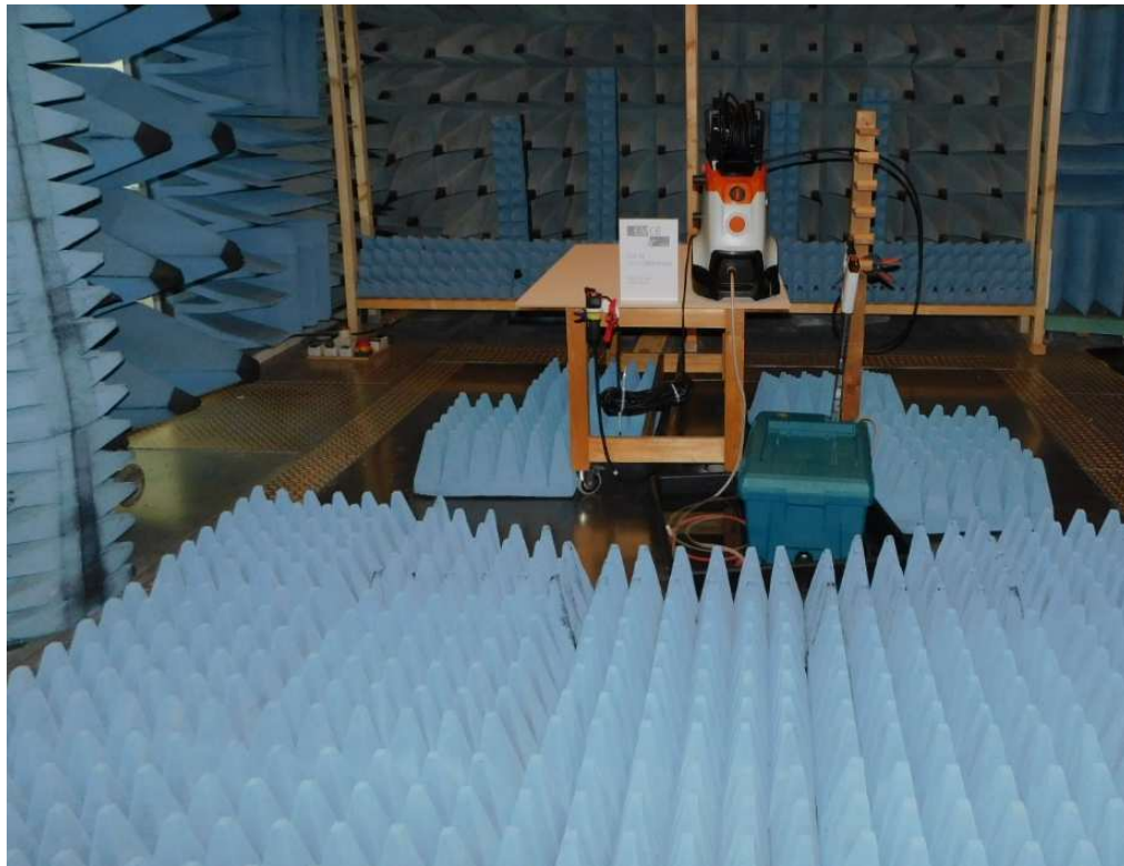
Final test setup – SAC [1 – 5 GHz]
