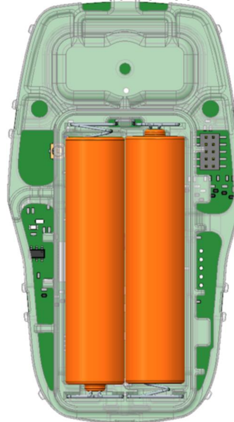
Back view transparent with batteries
