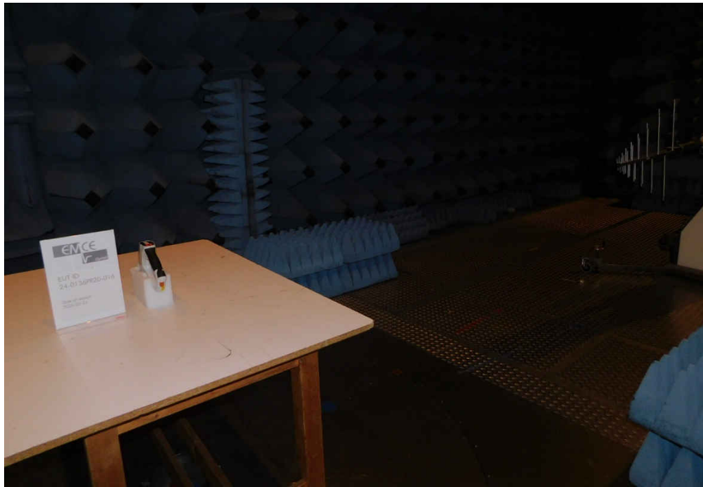
Pre-test setup – SAC [30 – 1000 MHz]
