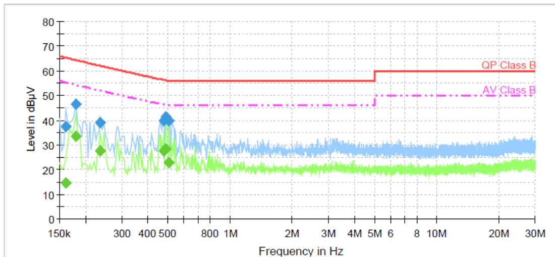
1.EMI Auto Test_2-Line Voltage LISN
