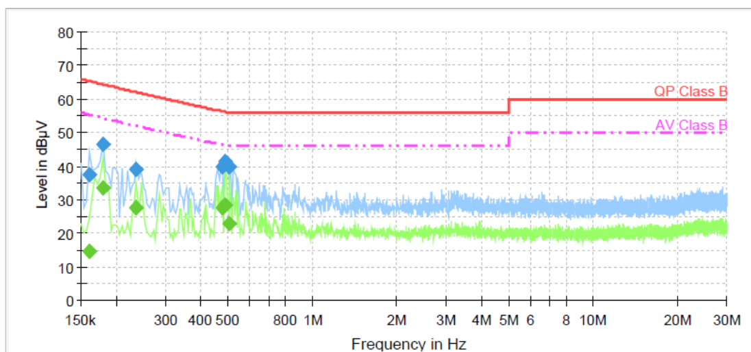
1.EMI Auto Test_2-Line Voltage LISN
