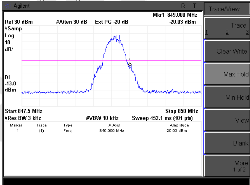
High Band Edge GSM 850 BAND CH 251
