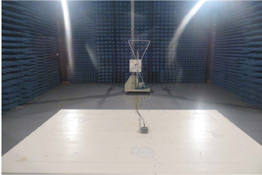
Photo of Radiated Emission Test Part 15.247
