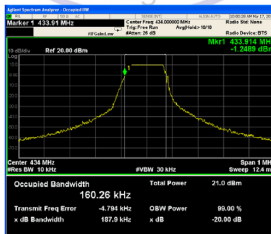
ASK Modulation
