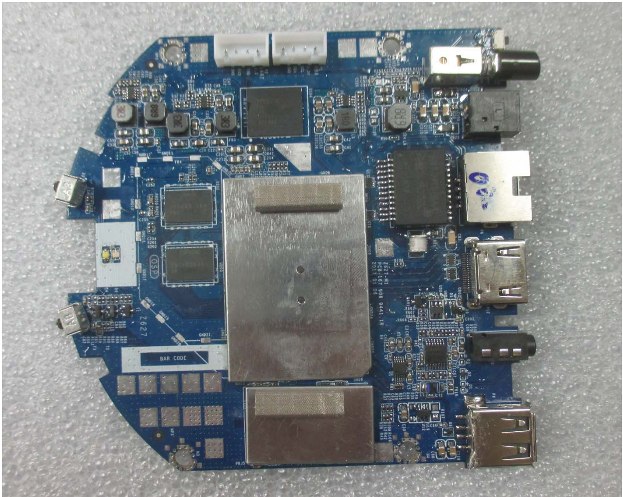
Fig. 7 PCB Board, Heat Sink Removed
