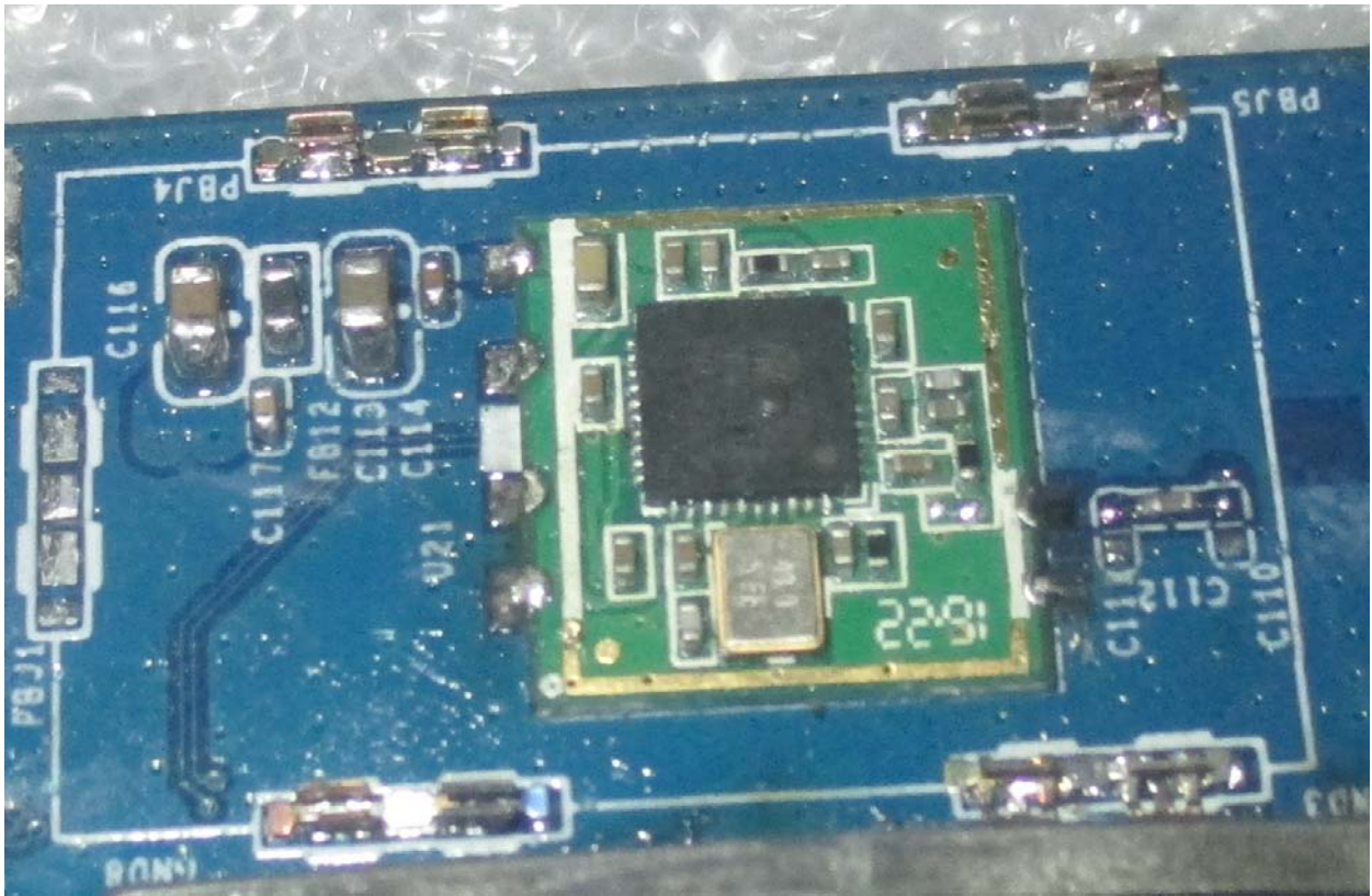
Fig. 10 WiFi Module PCB View
