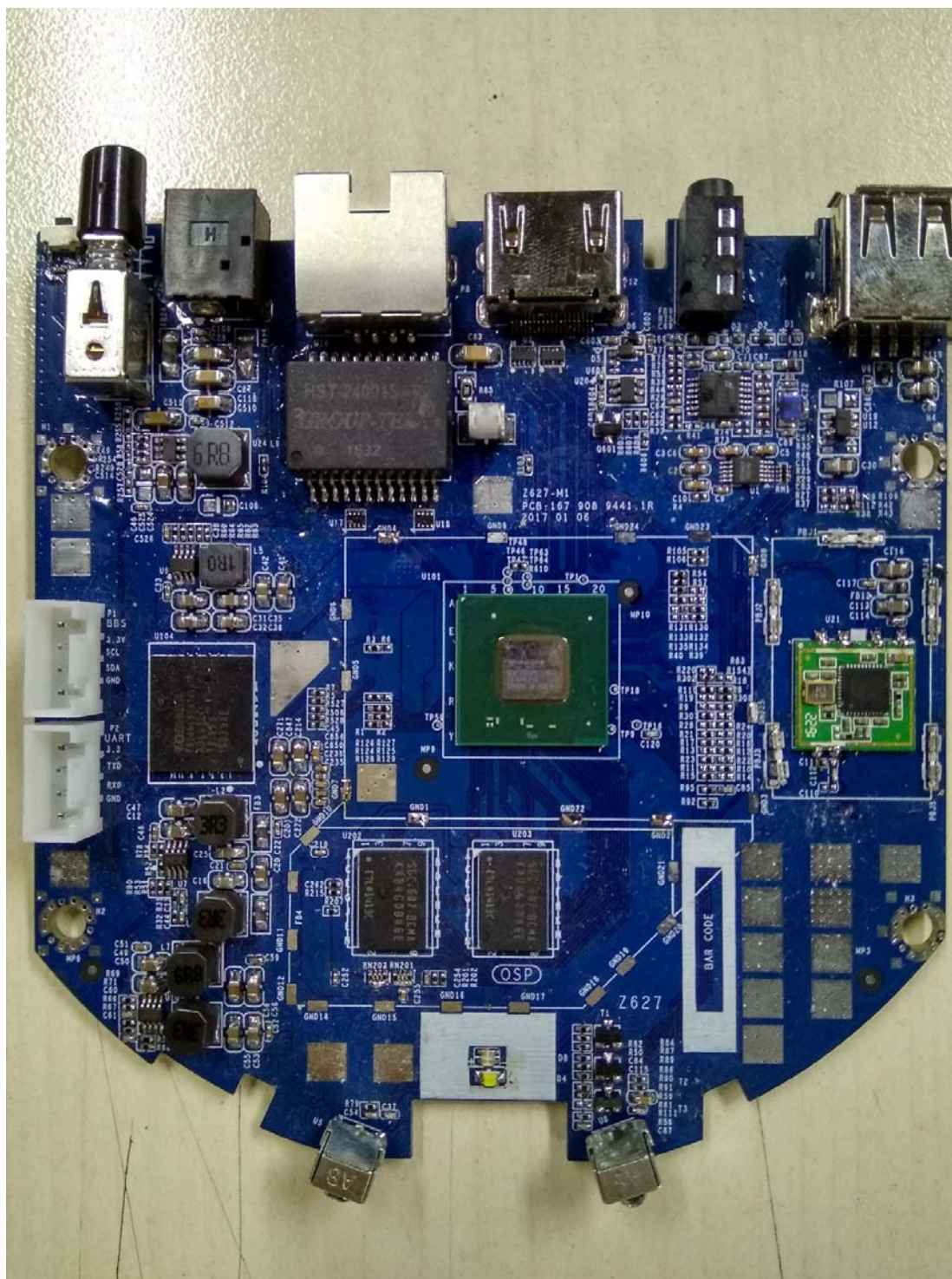
Fig. 8 PC Board, Removed CPU Cap & WIFI Module Cap.
