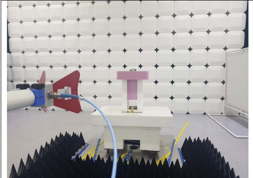
Radiated Emission_1 GHz ~ 10 GHz
