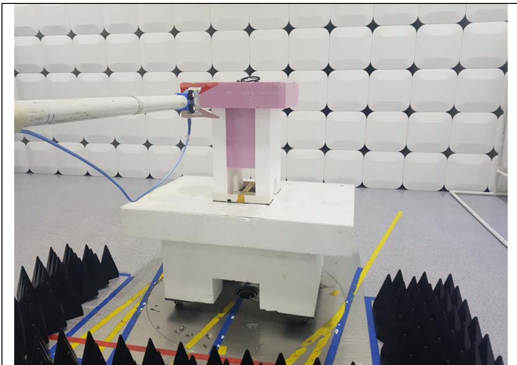
Radiated Emission_10 GHz ~ 18 GHz
