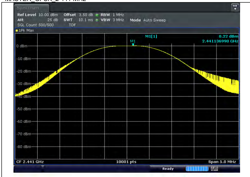
MASTER_GFSK 2 441 MHz
