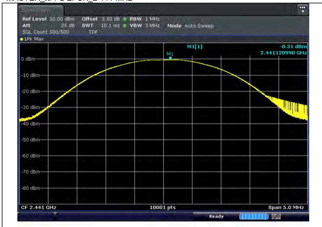
MASTER_π/4-DQPSK_2 441 MHz
