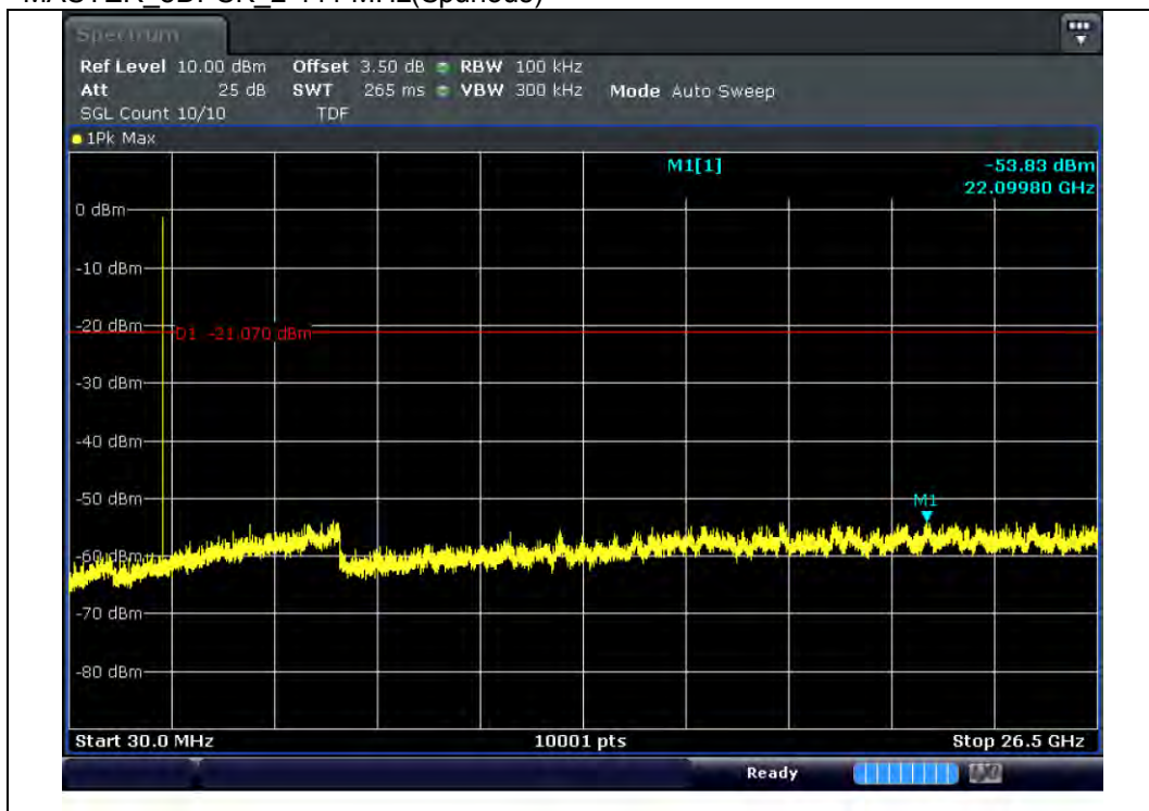
MASTER_8DPSK_2_441 MHz(Spurious)
