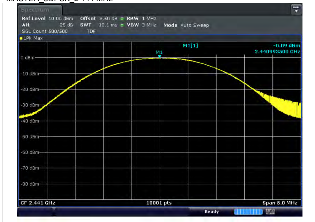
MASTER 8DPSK 2 441 MHz
