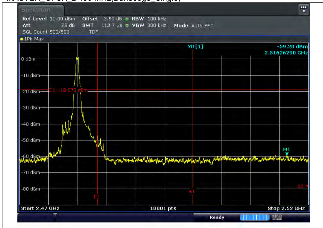
MASTER_GFSK_2 480 MHz(Bandedge_Single)
