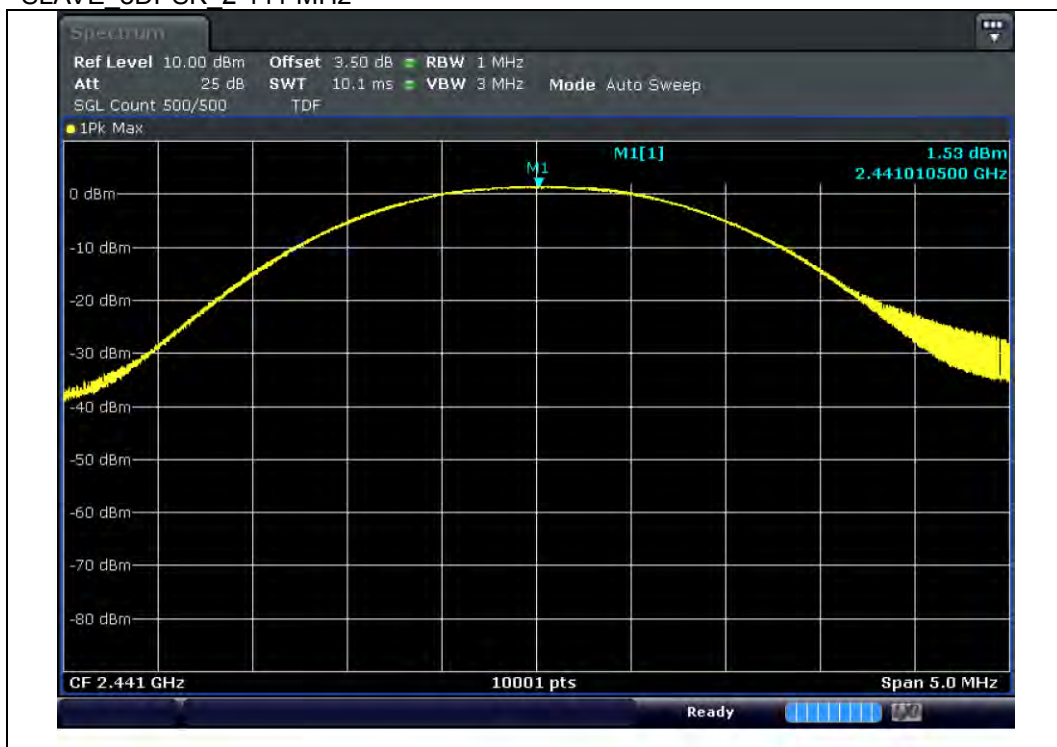
SLAVE 8DPSK 2 441 MHz
