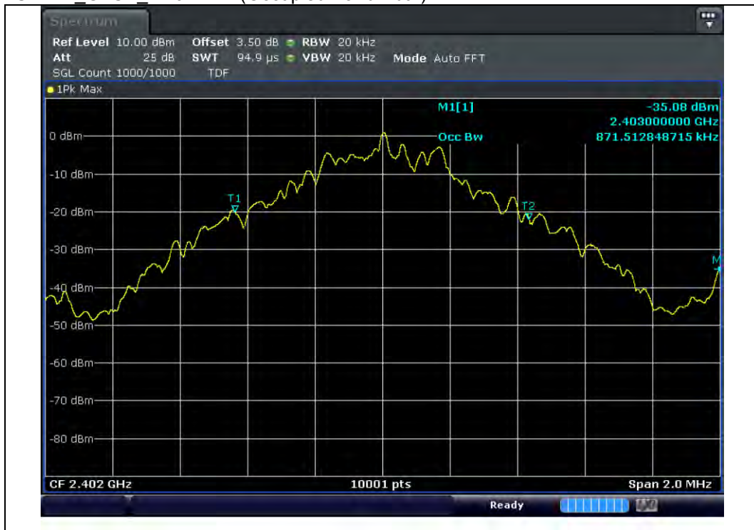
SLAVE_GFSK_2 402 MHz(Occupied Bandwidth)
