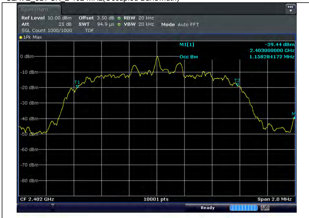
SLAVE_8DPSK_2 402 MHz(Occupied Bandwidth)
