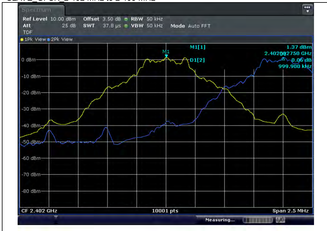
SLAVE_GFSK 2 402 MHz to 2 403 MHz
