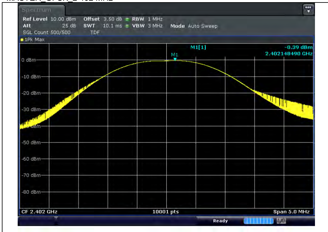
MASTER_GFSK 2 402 MHz
