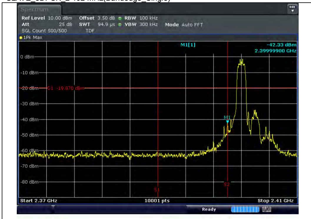
SLAVE_8DPSK_2 402 MHz(Bandedge_Single)
