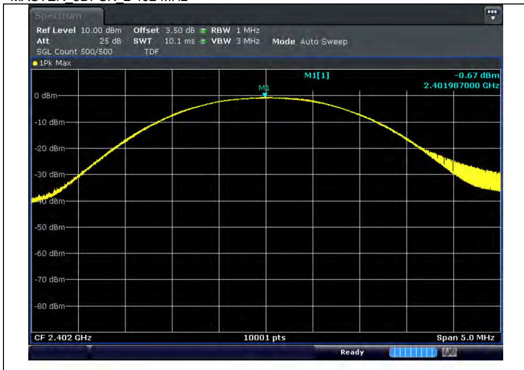
MASTER 8DPSK 2 402 MHz
