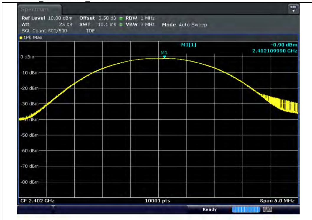
MASTER_π/4-DQPSK_2 402 MHz
