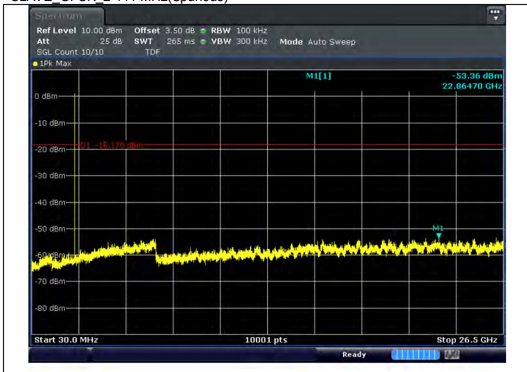
SLAVE_GFSK_2 441 MHz(Spurious)
