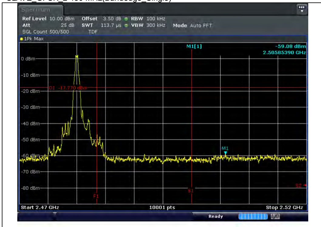
SLAVE_GFSK 2 480 MHz(Bandedge_Single)
