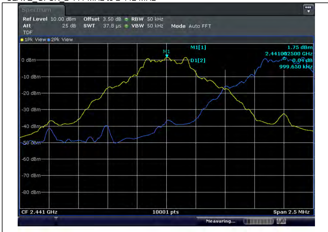
SLAVE_GFSK 2 441 MHz to 2 442 MHz
