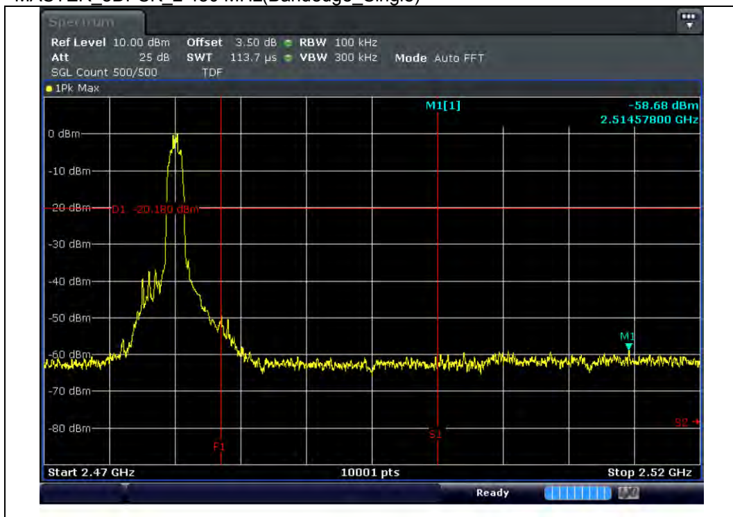
MASTER_8DPSK_2_480 MHz(Bandedge_Single)
