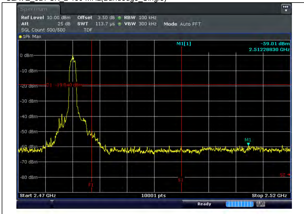
SLAVE_8DPSK_2 480 MHz(Bandedge_Single)
