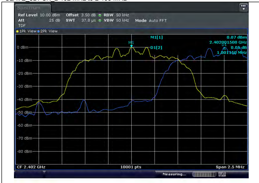
SLAVE_8DPSK 2 402 MHz to 2 403 MHz
