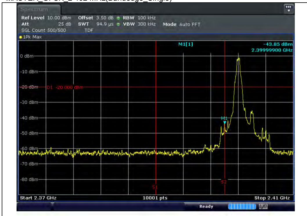
MASTER_GFSK_2 402 MHz(Bandedge_Single)
