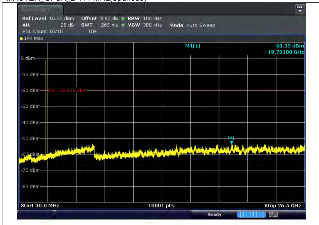
MASTER_GFSK_2_441 MHz(Spurious)
