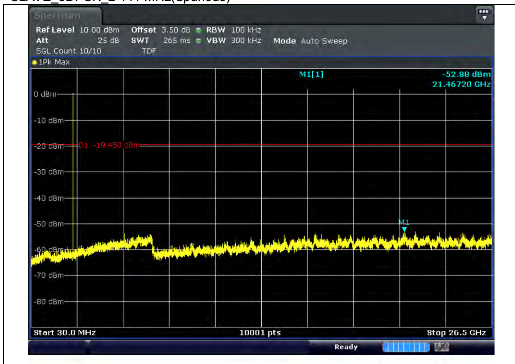
SLAVE_8DPSK_2.441 MHz(Spurious)
