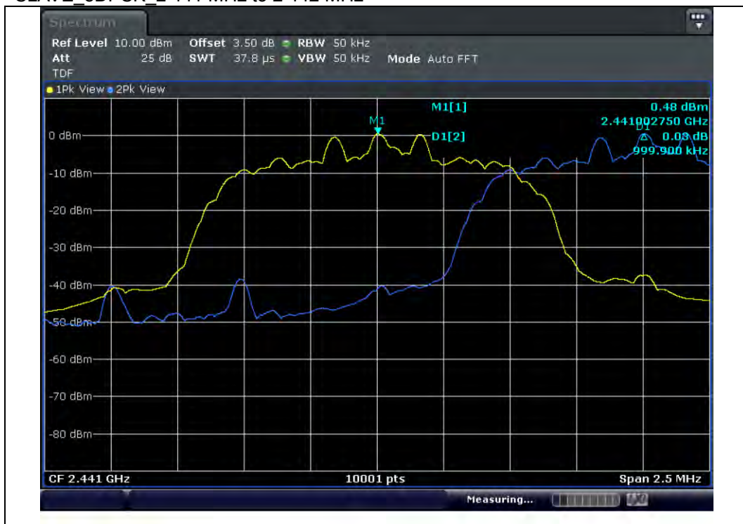
SLAVE_8DPSK 2 441 MHz to 2 442 MHz
