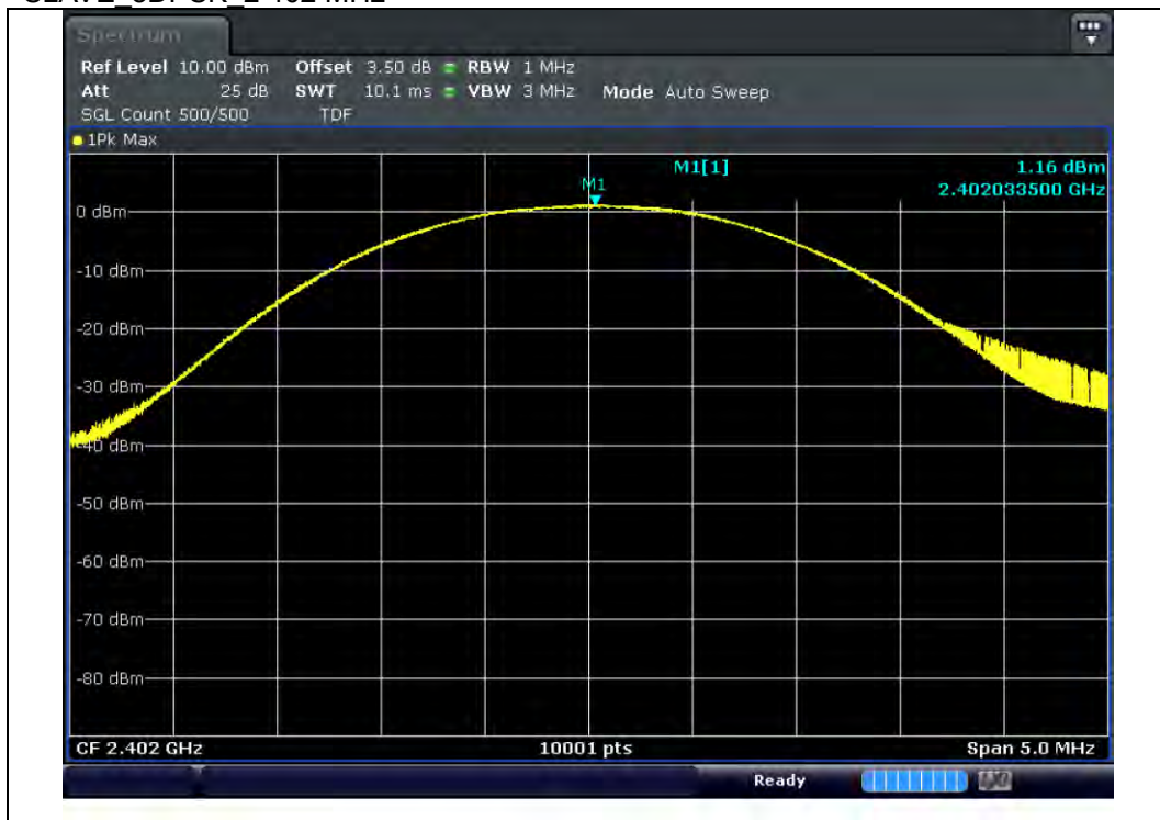
SLAVE 8DPSK 2 402 MHz
