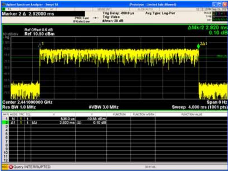
Pi/4DQPSK 2DH5 Middle Channel
