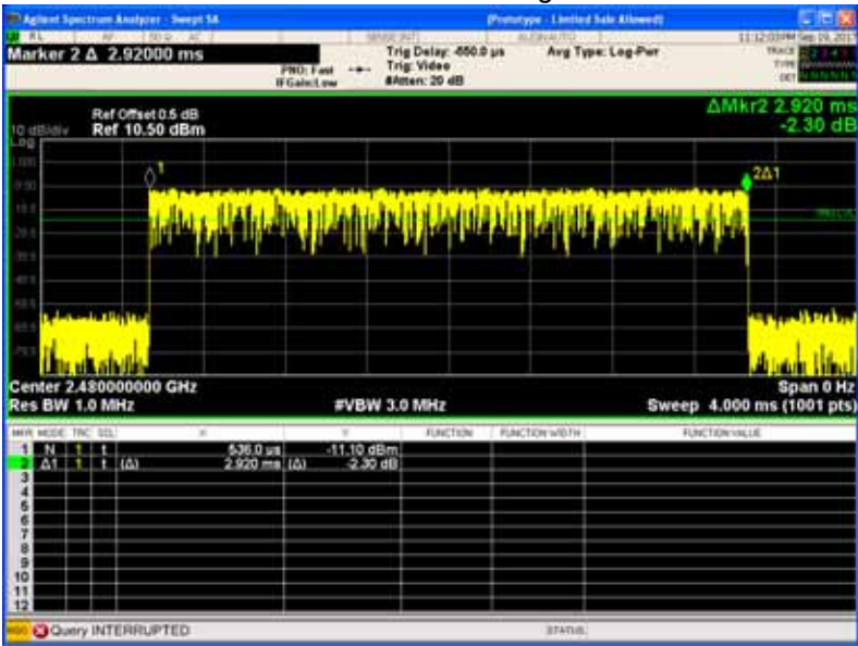
Pi/4DQPSK 2DH5 High Channel
