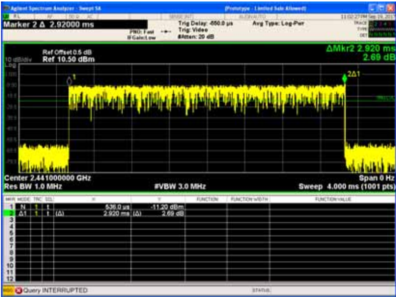
8DPSK 3DH5 Middle Channel
