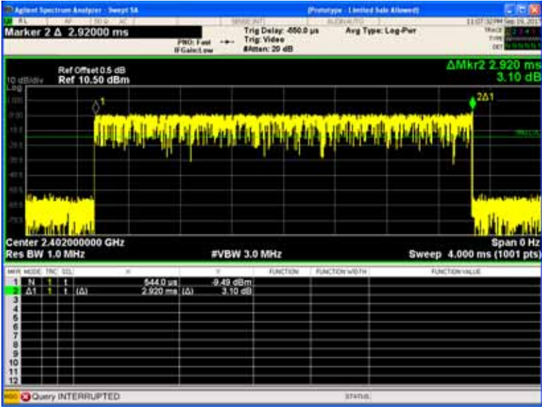
Pi/4DQPSK 2DH5 Low Channel
