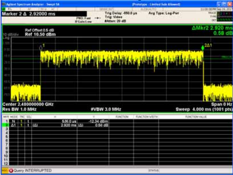
8DPSK 3DH5 High Channel
