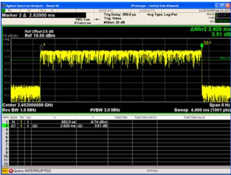
8DPSK 3DH5 Low Channel
