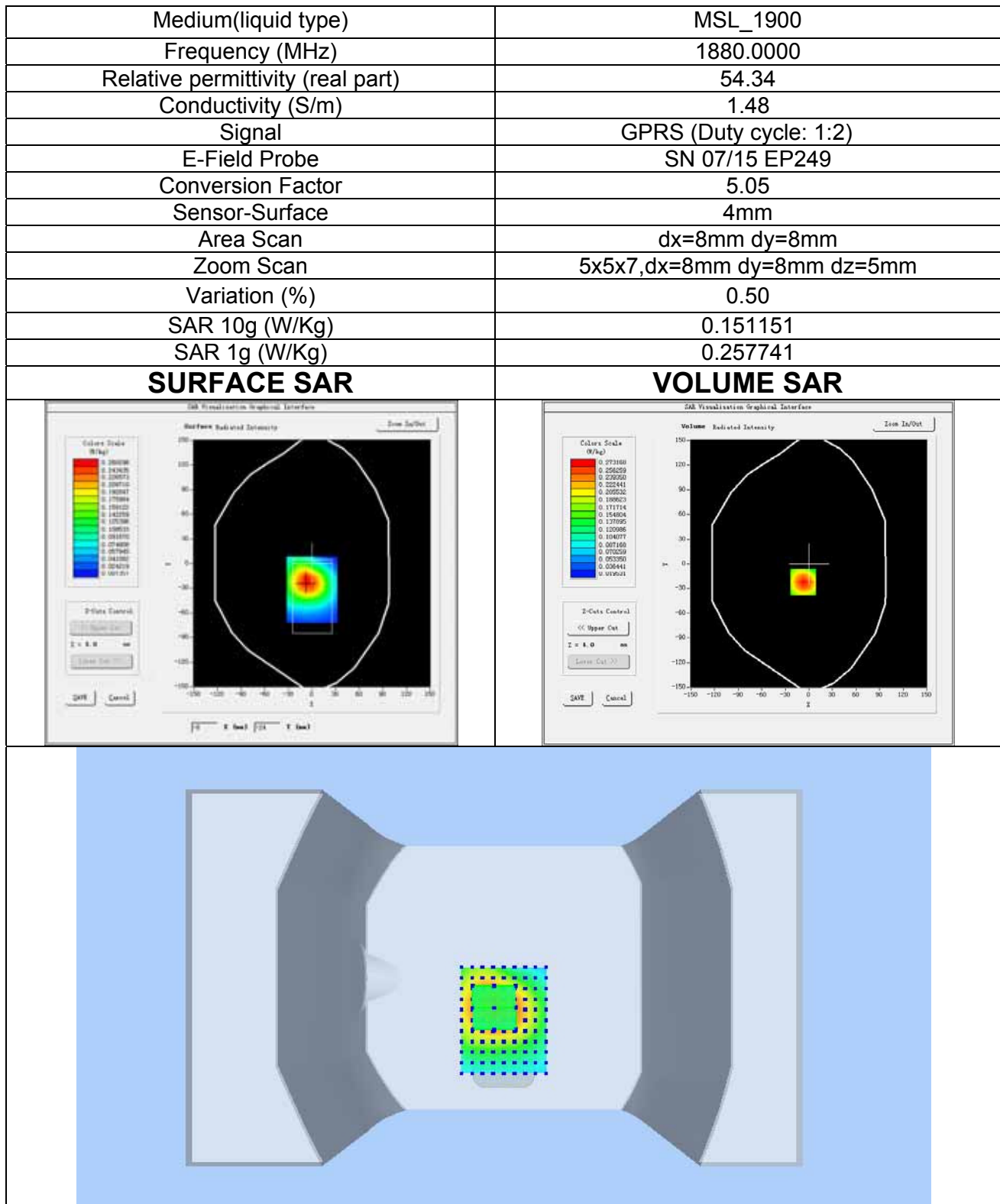
Plot 14: GPRS1900, Middle channel (Body-worn, Front Surface) Product Description: Mobile Phone Test Date: Apr 13,2017
