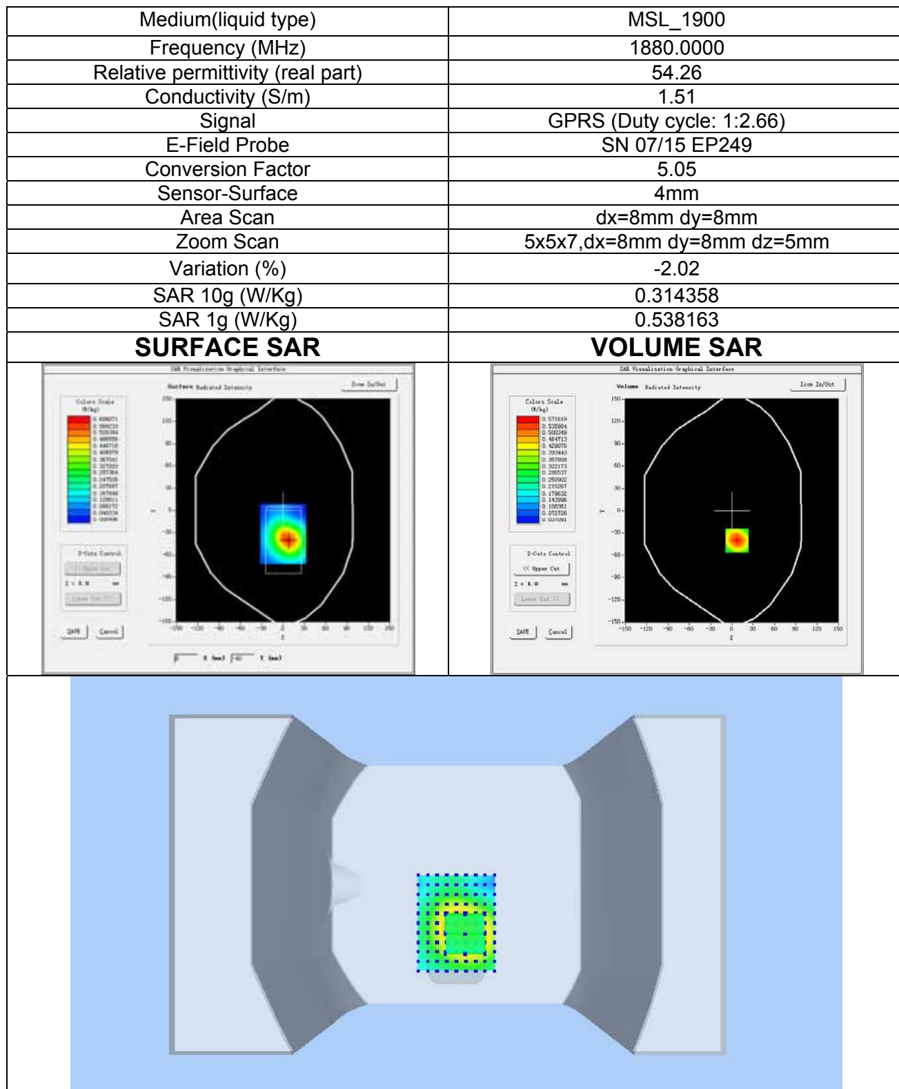
Plot 14: GPRS1900, Middle channel (Body-worn, Front Surface) Product Description: Mobile Phone Test Date: Apr 14,2017
