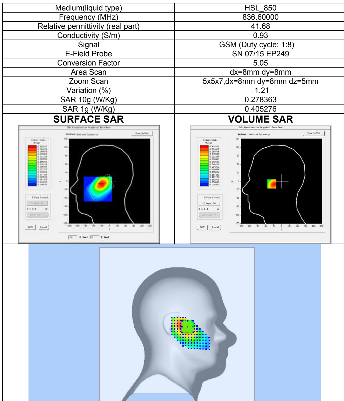
Plot 4: GSM850MHz, Middle channel (Left Head , Tilt) Product Description: Mobile Phone Test Date: Apr 18, 2017
