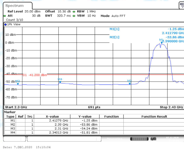
11B_Ant1_Low_2412_Peak
