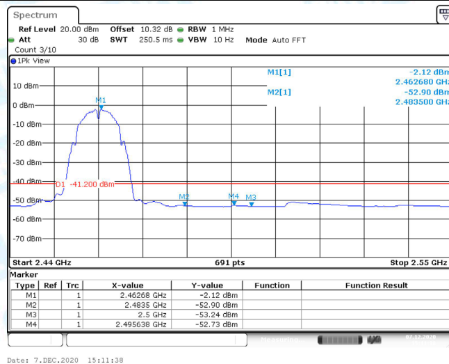
11B_Ant1_High_2462_AV
