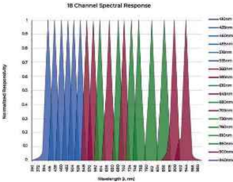
18 wavelengths throughout the UV - VIS - IR range are covered by sensors used by the PrimeLab 2.0. Narrow peaks on the spectral curve allow utmost accuracy.
