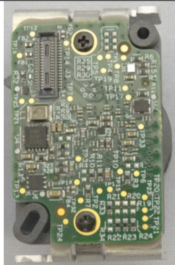
Bottom side of camera sensor PCB
