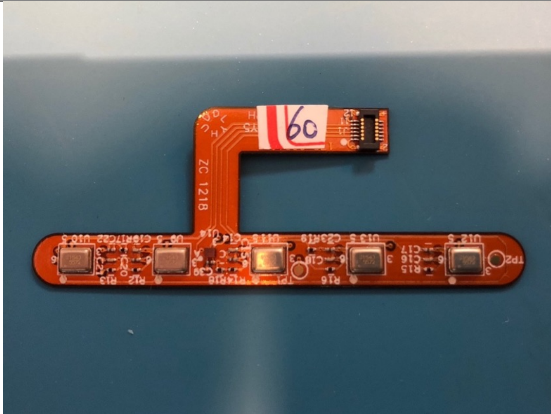
Top side of microphone array FPC
