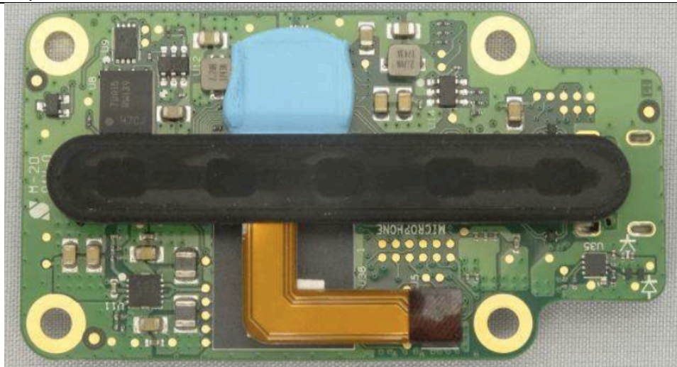
Bottom side of mainboard PCB with microphone FPC
