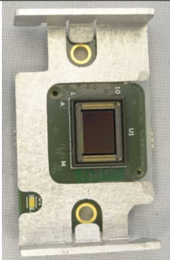
Top side of camera sensor PCB
