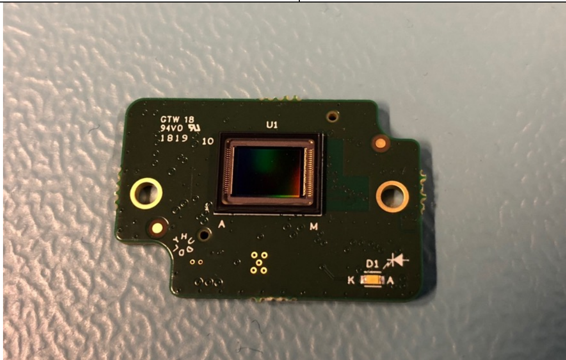
Top side of camera sensor PCB – without cover
