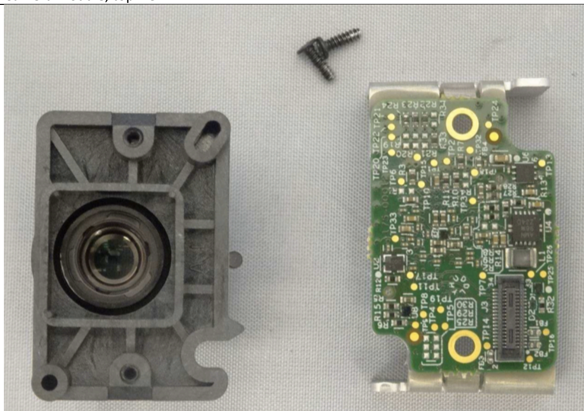
Camera module, disassembled
