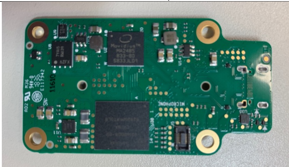
Bottom side of mainboard PCB – without microphone FPC
