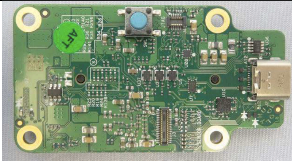
Top side of mainboard PCB
