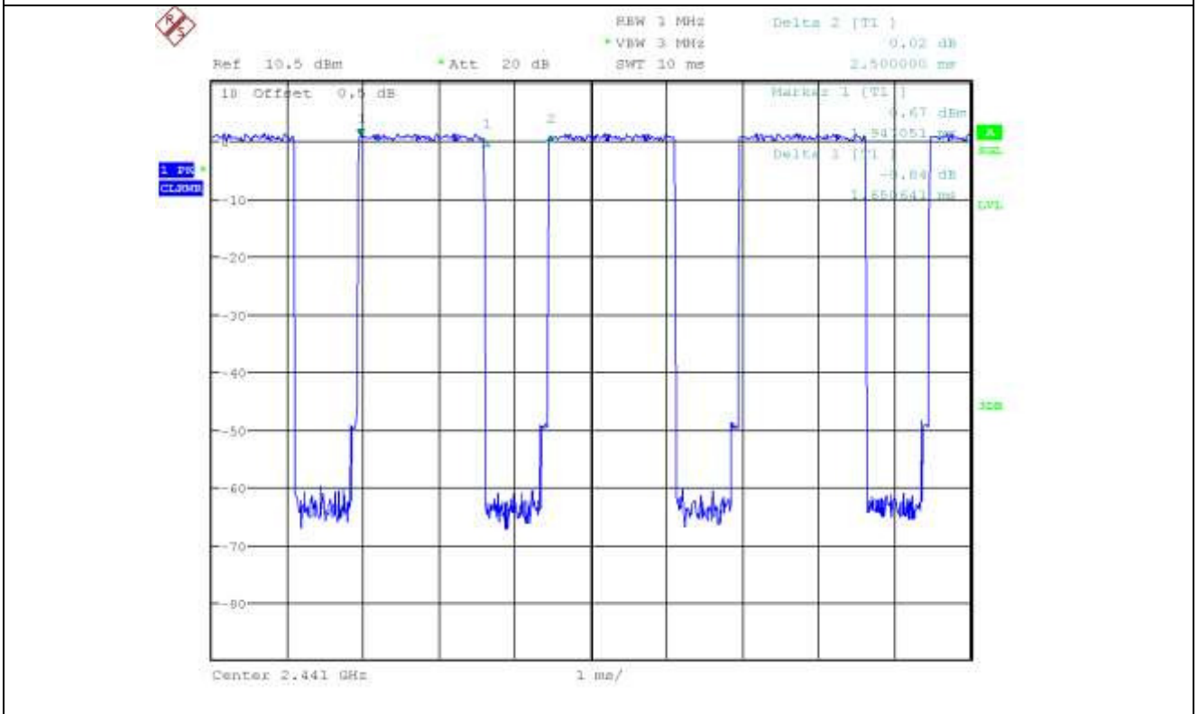
3-DH3
