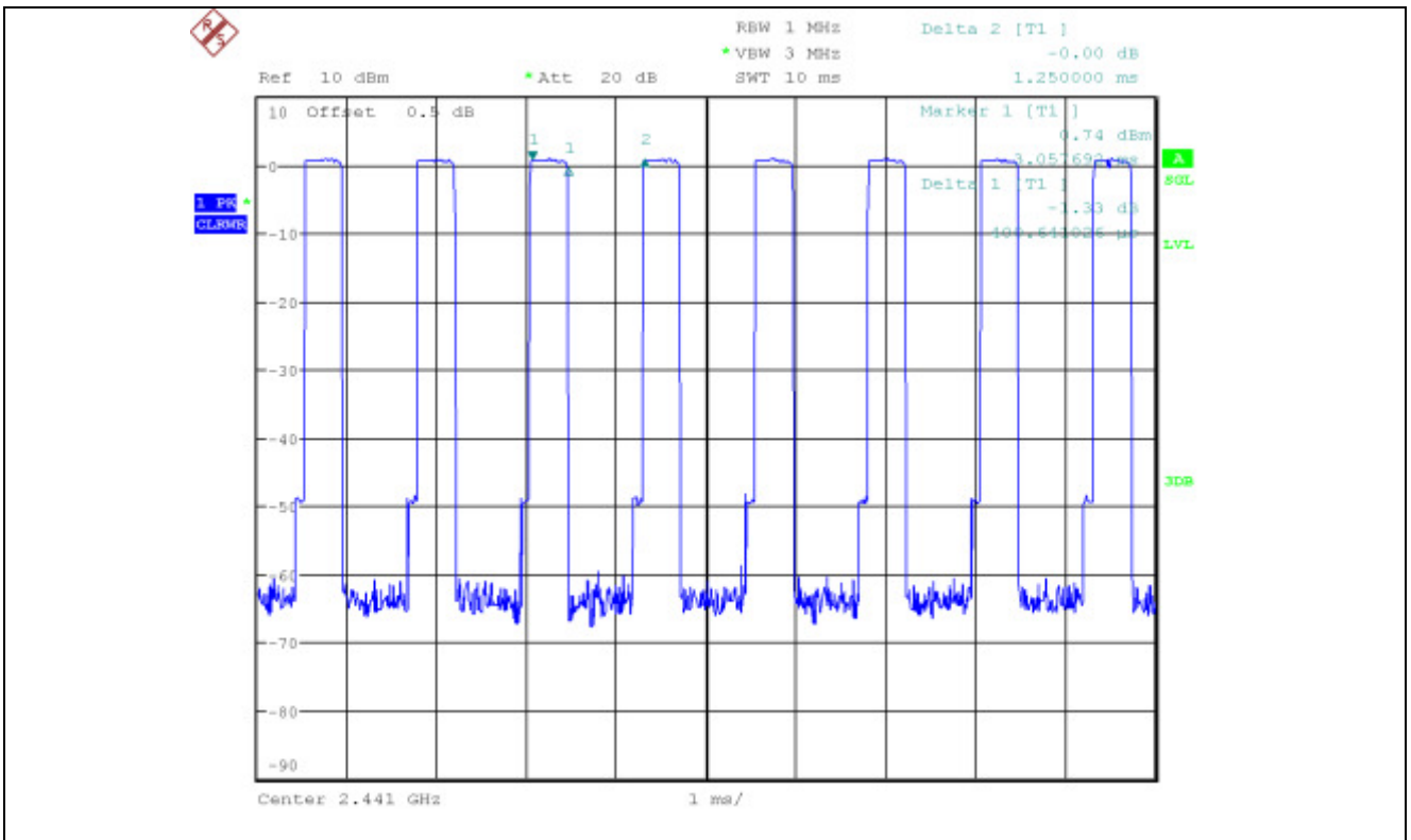
2-DH1
