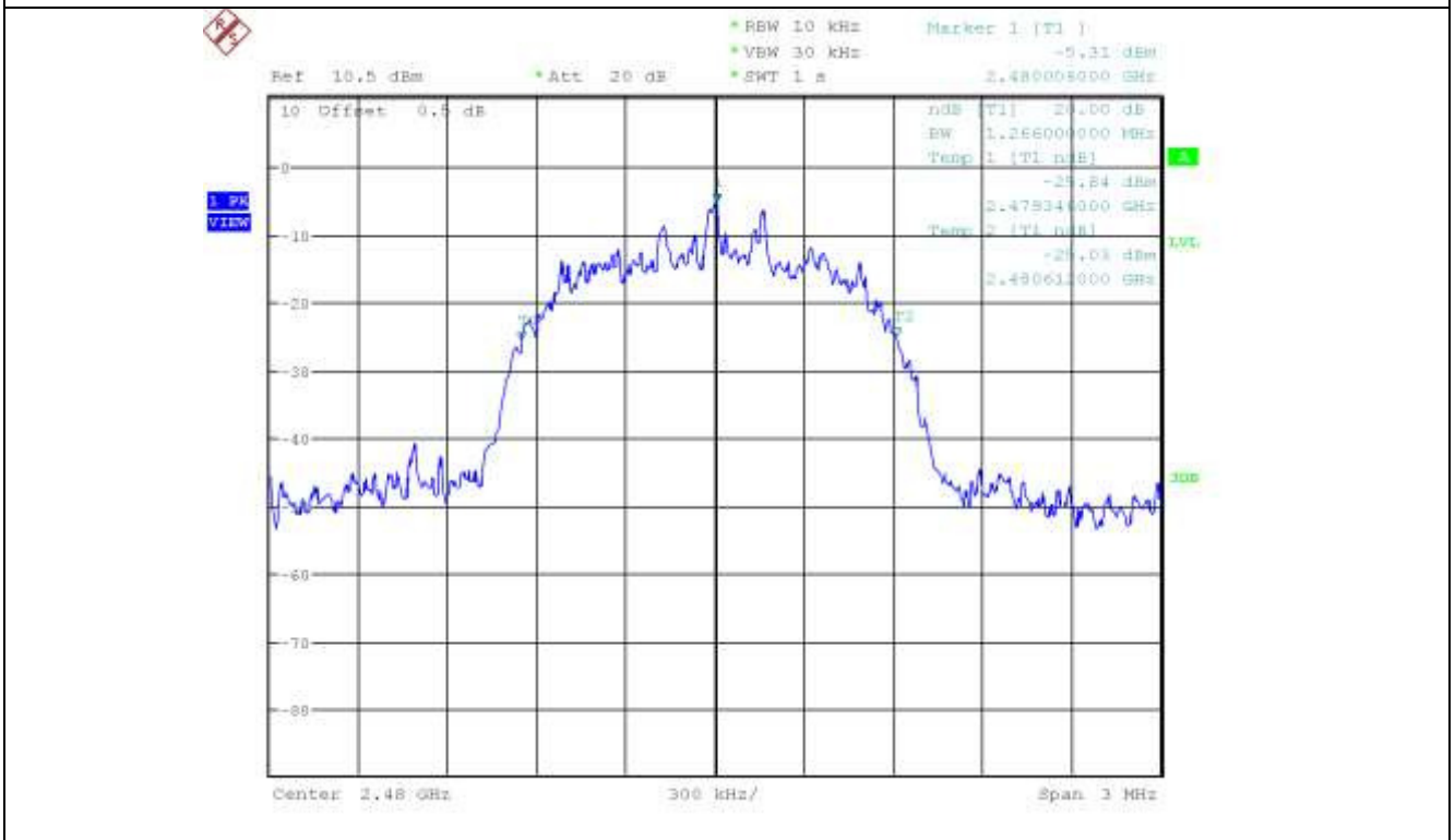
High Channel
