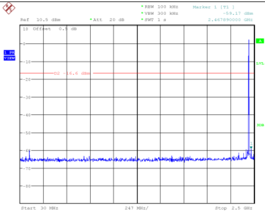
Middle Channel
