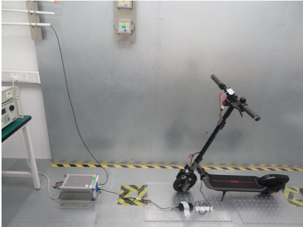
Description: Rear View of AC Conducted Emissions Test Setup
