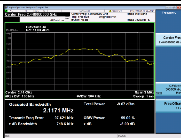
Channel 19 (2440MHz)
