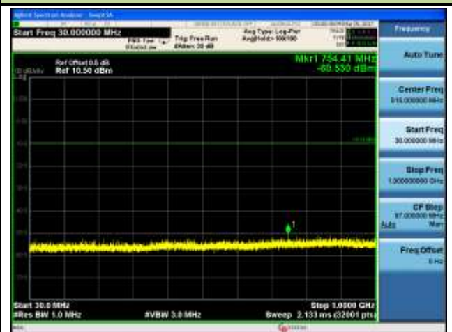
CH39 (2441MHz) DH5(1Mbps)
